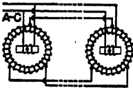
Selsyn-motor circuit for single-phase a-c line.
